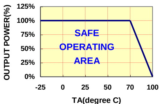
DERATING CURVES
