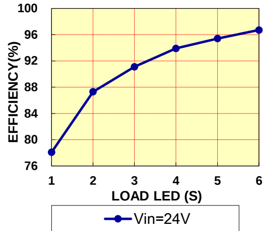
EFFICIENCY VS. LOAD LED 0.35A
