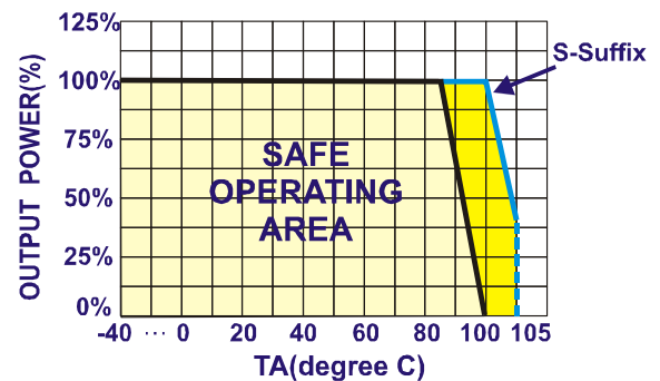
TEMPERATURE DERATING
