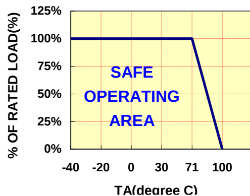
DERATING CURVE
