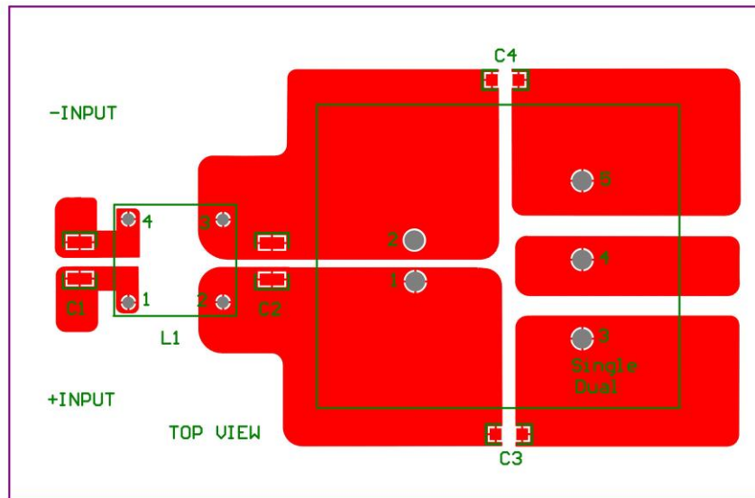
Recommended EN55032 Class B Filter Circuit Layout
