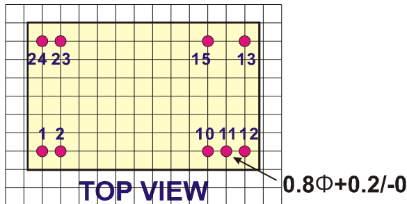
PACKAGE "C"
