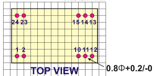
PACKAGE "D"
