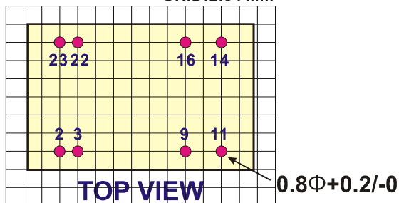
PACKAGE "P"
