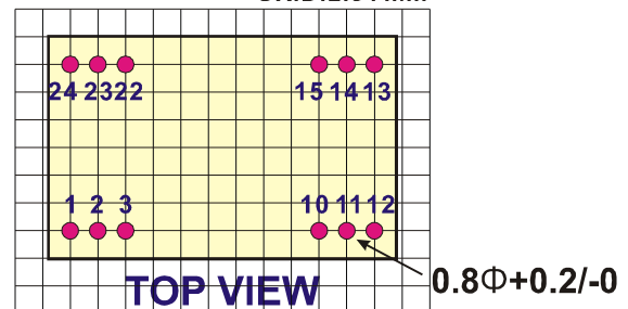
PACKAGE "T"
