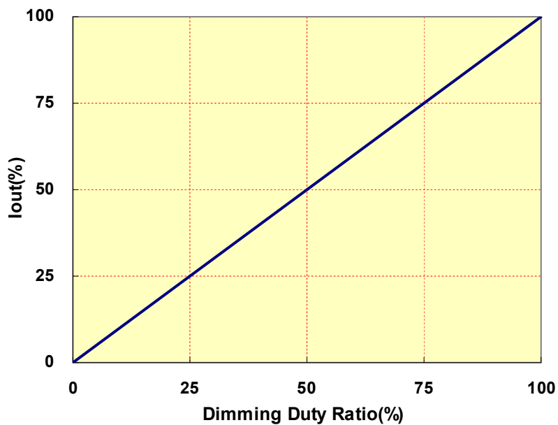
Fig.1 Dimming Duty Cycle:0%-100%
